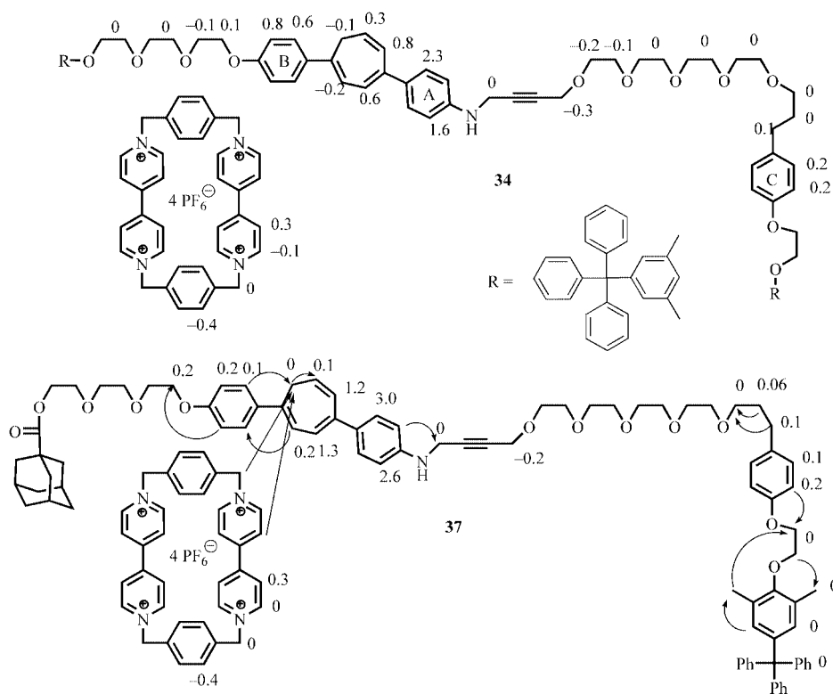
Scheme 18. CIS values of proton resonances of rotaxanes 34 and 37 obtained by comparison of the proton resonances of uncomplexed molecular threads and compound 2 with related proton resonances measured in the rotaxanes. Arrows mark NOEs between protons observed by ROESY spectra.
