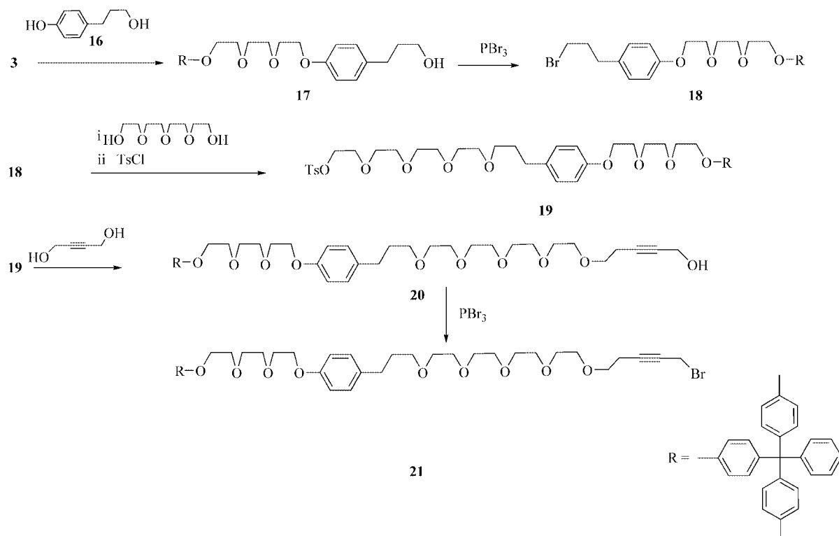
Scheme 9. Synthesis of the eastern half of the molecular thread of rotaxane 22 .
