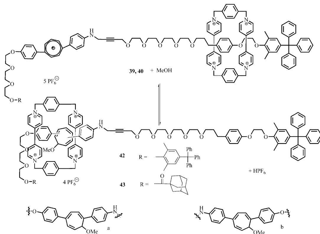
Scheme 21. Reaction of the tropylium rotaxanes with methanol and the most probable isomers.
