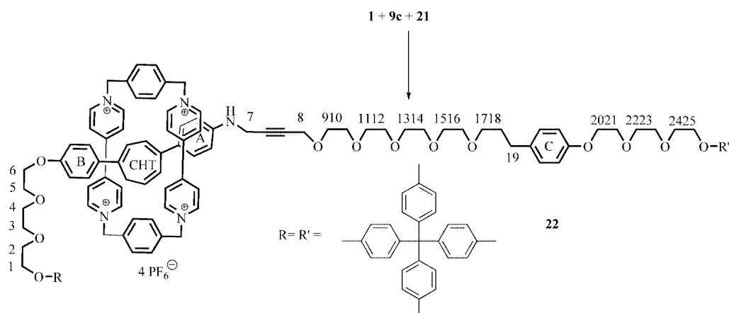
Scheme 10. Synthesis of rotaxane 22 .
