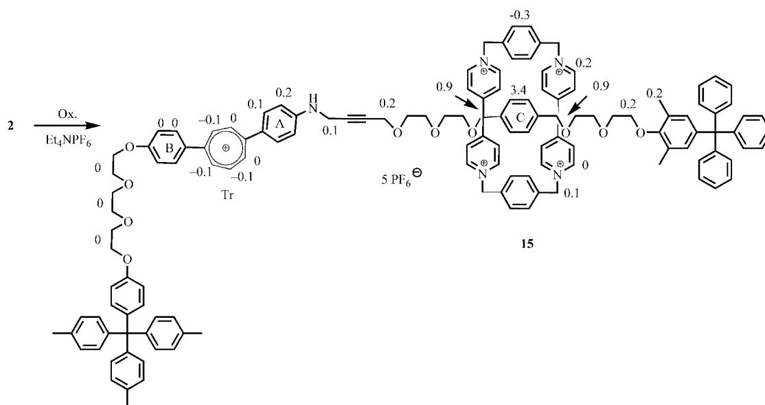
Scheme 8. CIS values of some protons of rotaxane 15 calculated by comparison of related protons of molecular thread 41 (for the tropylium ion region) and of 14 (for the region of station C).
