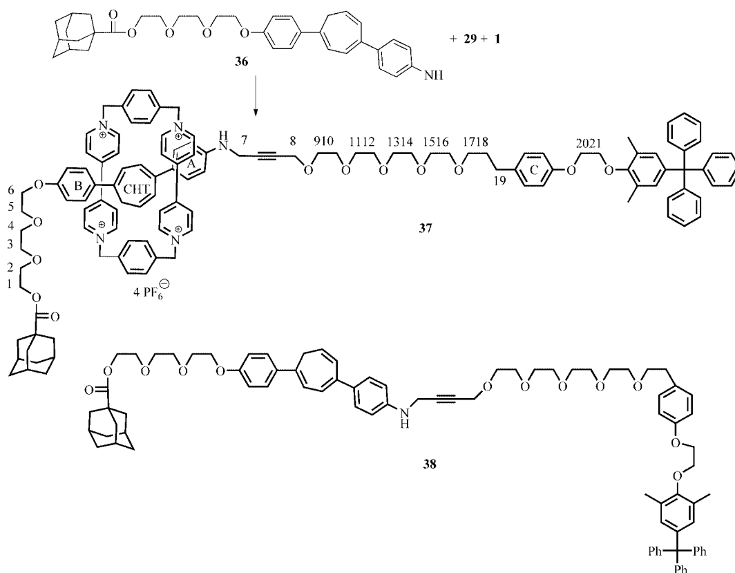
Scheme 17. Synthesis of rotaxane 37 .
