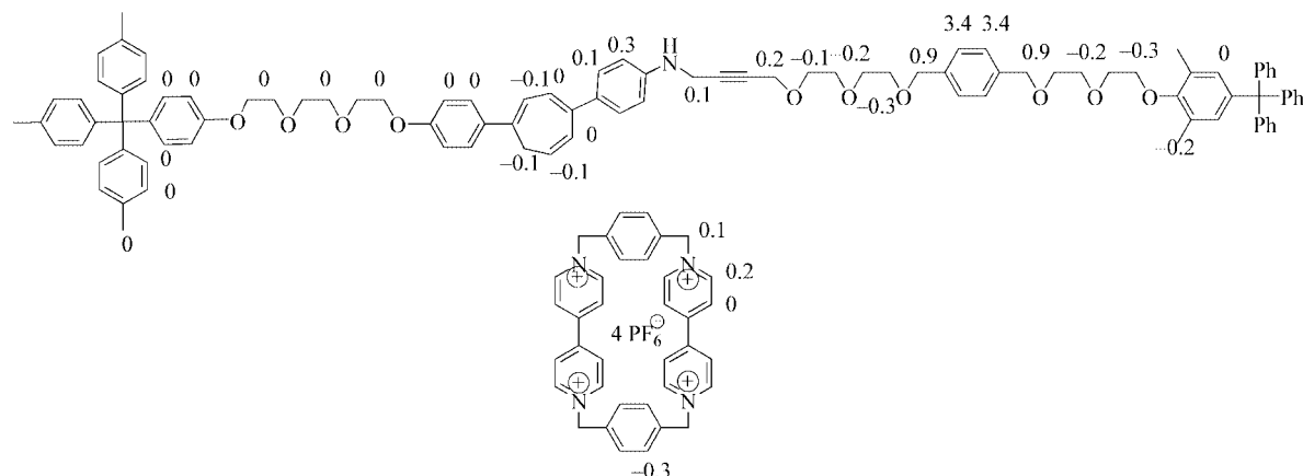
Scheme 6. Chemically-induced shift (CIS) of some proton resonances of rotaxane 2 calculated by comparison of related proton signals of fragments of the uncomplexed molecular thread and of rotaxane 2 ( \delta_{9c-\delta 2} and \delta_{14-\delta 2} ), and of the uncomplexed ring 1 and 2 .
