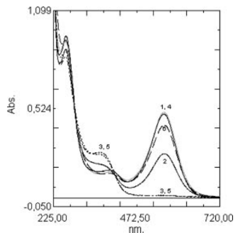
Figure 3. UV/Vis absorption spectra of rotaxane 42 : 1 – rotaxane 39 in acetonitrile solution; 2 – after addition of methanol (0.5 mL/9.5 mL); 3 – after addition of \text{NaHCO}_3 ; 4 – addition of TFA; 5 – addition of \text{NaHCO}_3 ; 6 – after addition of TFA.
