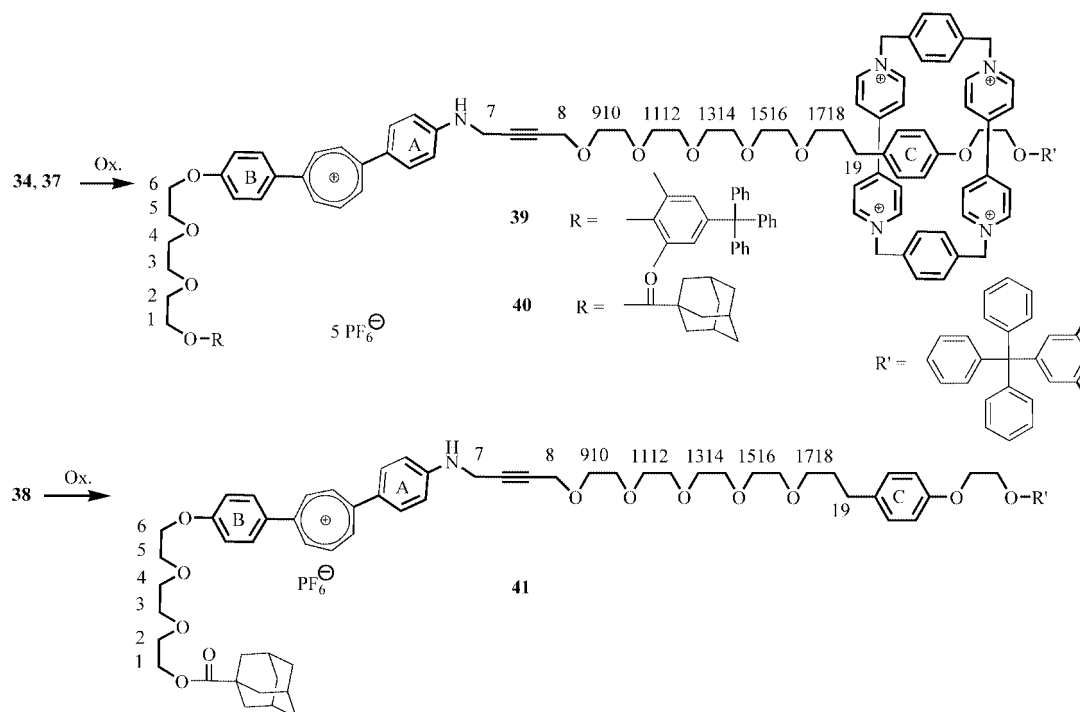
Scheme 19. Electrochemical oxidation of rotaxanes 34 and 37 and molecular thread 38 .
