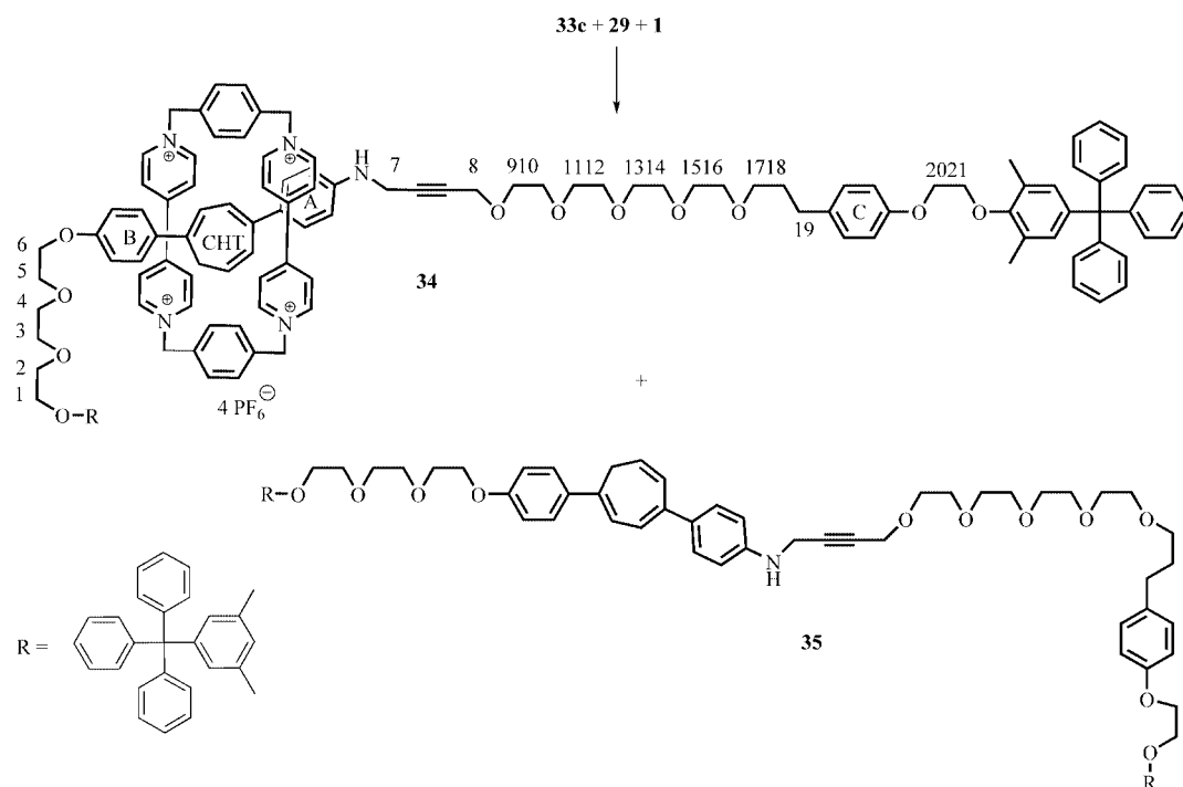
Scheme 16. Synthesis of rotaxane 34 .
