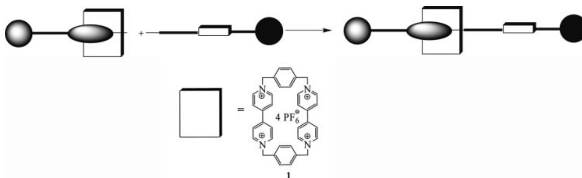
Scheme 3. Principle of rotaxane synthesis.
