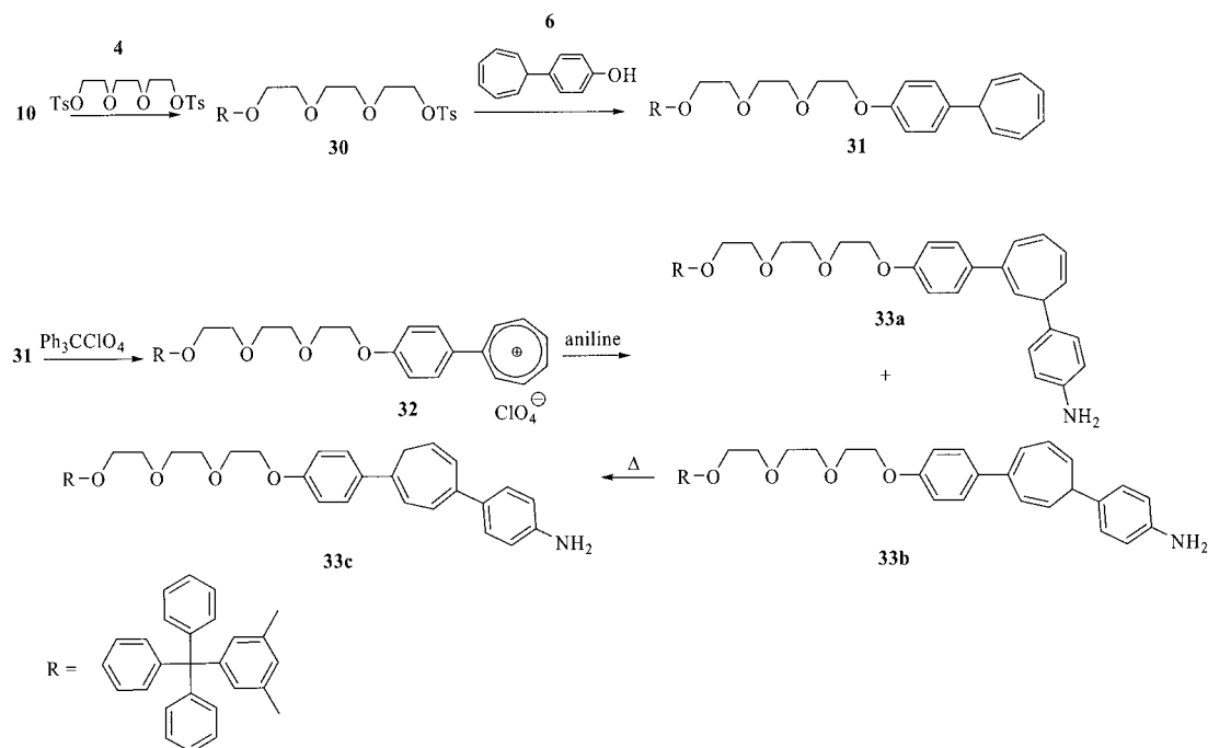
Scheme 15. Synthesis of the western half of the molecular thread of rotaxane 34 .
