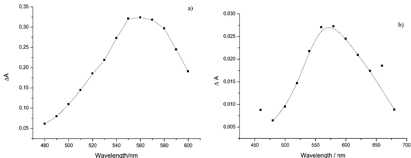
Figure 2. a) Transient absorption spectra observed during flash photolysis of molecular thread 44 . b) Transient absorption spectra observed during flash photolysis of rotaxane 43 .
