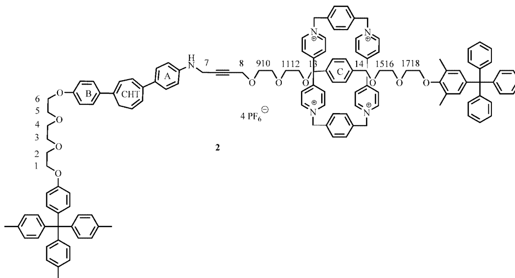
Scheme 2. Rotaxane 2 with numbering of some atoms.
