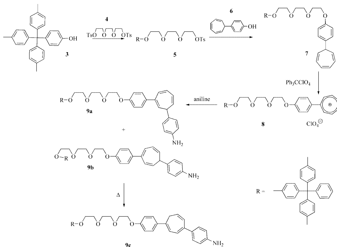
Scheme 4. Synthesis of the western half of the molecular thread.
