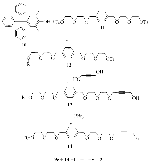
Scheme 5. Synthesis of the eastern half of the molecular thread.
