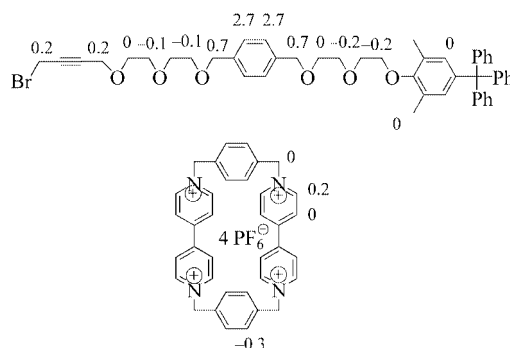
Scheme 7. CIS values of the protons of the pseudorotaxane 1/14 calculated by comparison of the uncomplexed and complexed components.
