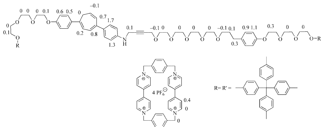
Scheme 11. CIS values obtained for rotaxane 22 .
