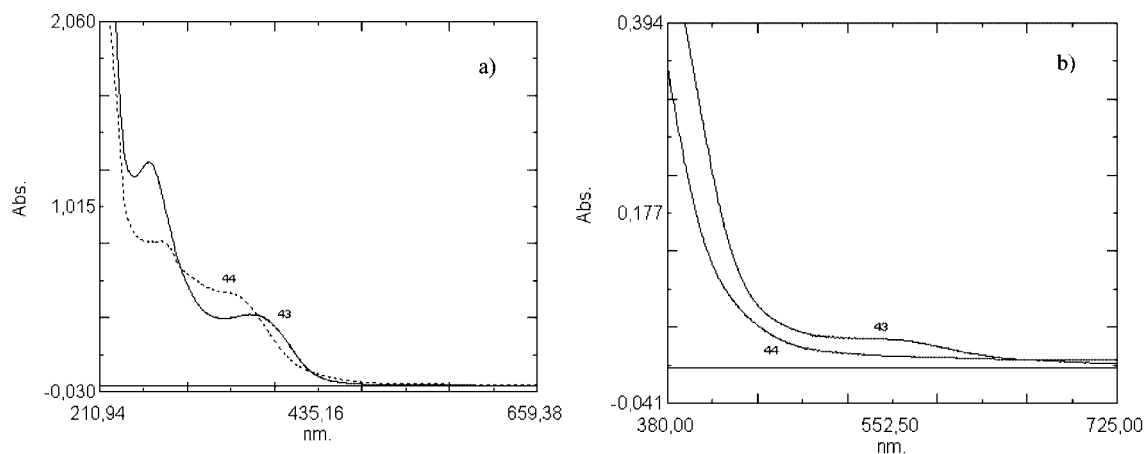
Figure 1. a) UV/Vis absorption spectra of rotaxane 43 ( 2.5 \times 10^{-5} M) and molecular thread 44 ( 3 \times 10^{-5} M) in acetonitrile solution containing methanol (1 M). b) Partial UV/Vis-absorption spectra of rotaxane 43 ( 5 \times 10^{-4} M) and molecular thread 44 ( 5 \times 10^{-4} M) in acetonitrile solution containing methanol (1 M).
