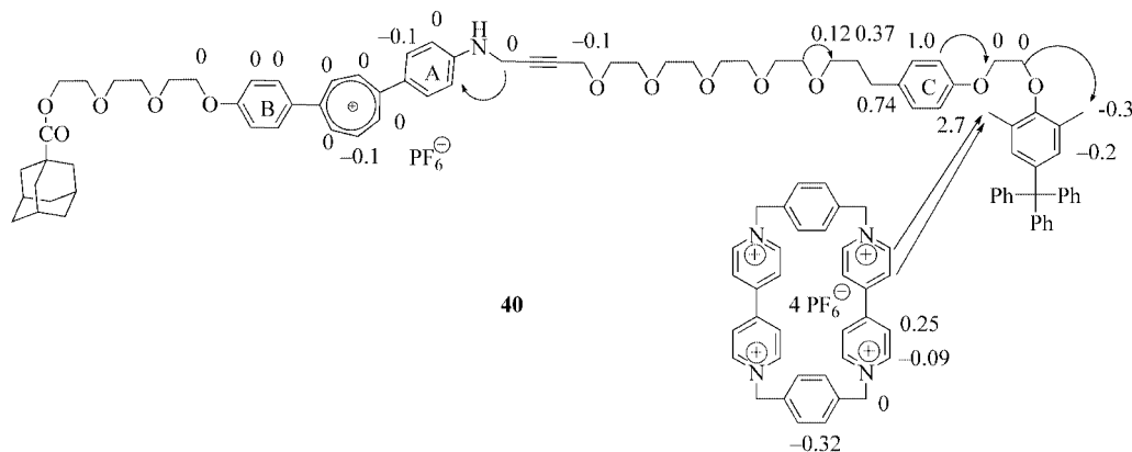
Scheme 20. CIS values calculated for rotaxane 40 . Arrows mark NOEs between protons observed by ROESY spectra.
