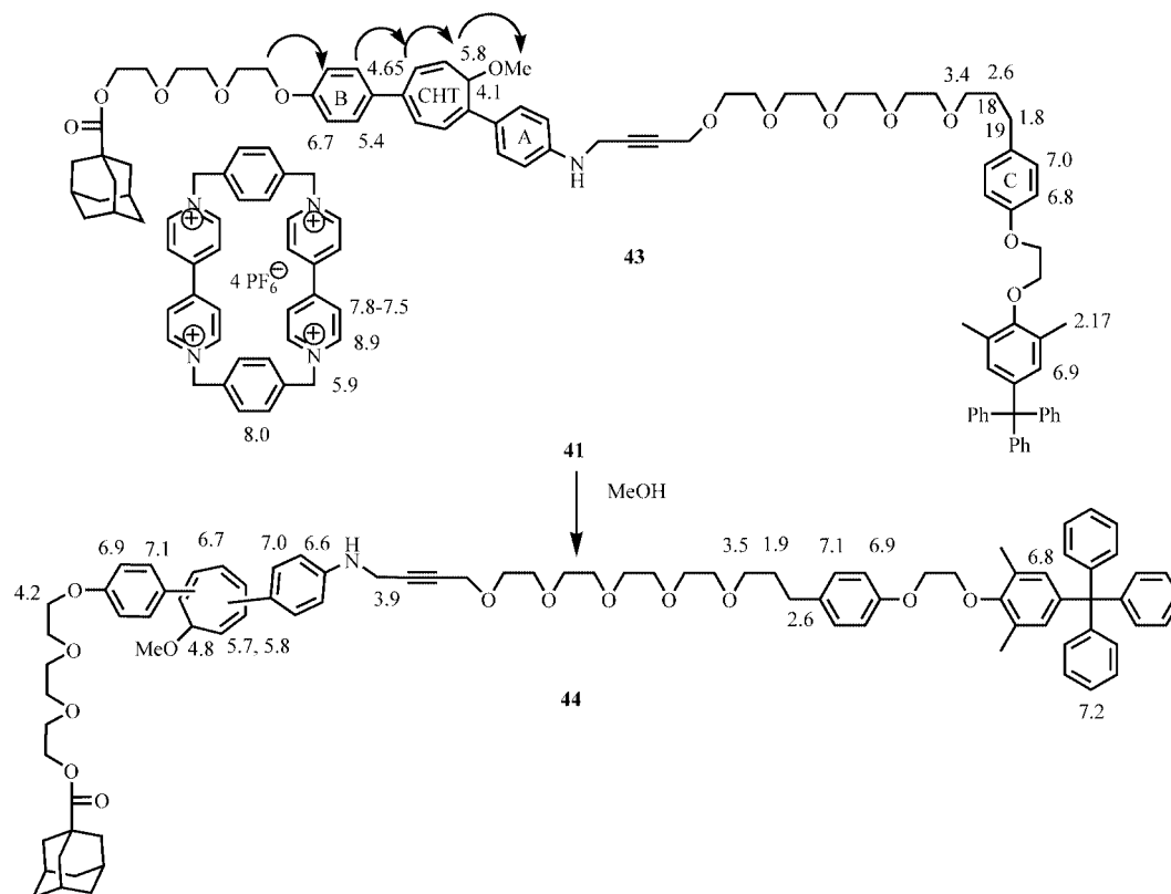
Scheme 22. Some proton resonances of rotaxane 43 and thread 44 . Arrows mark NOEs between protons observed by ROESY spectra.
