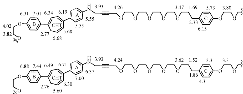
Scheme 12. Proton resonances of the two conformers of rotaxane 22 ( \delta , [D 6 ]acetone solutions).
