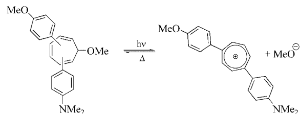
Scheme 1. Principle of photoheterolysis of a methoxy-diarylcycloheptatriene.
